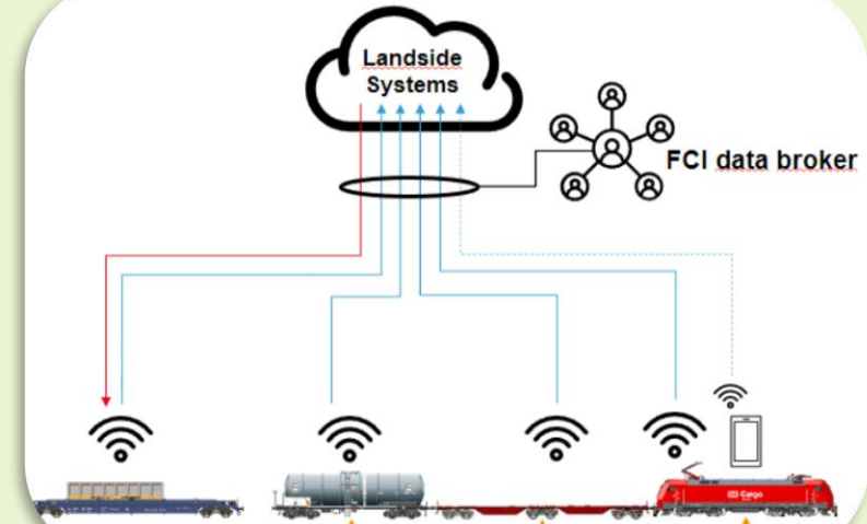
DAC/FDFTO Proposed Architecture
